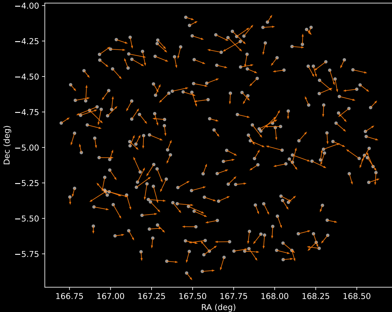
GALAH DR4 Cluster 2 Proper Motion Vectors (n=216)
