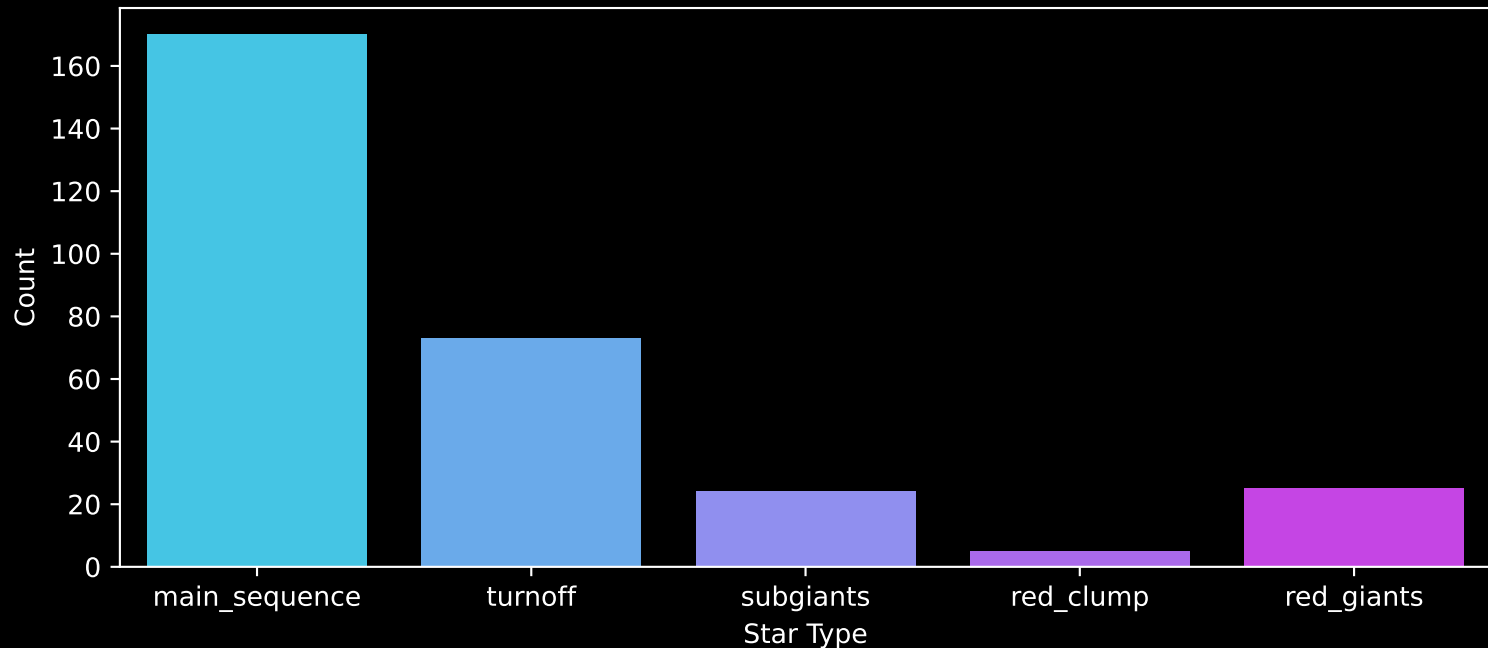
GALAH DR4 Field: [697] Count plot of Star Type
