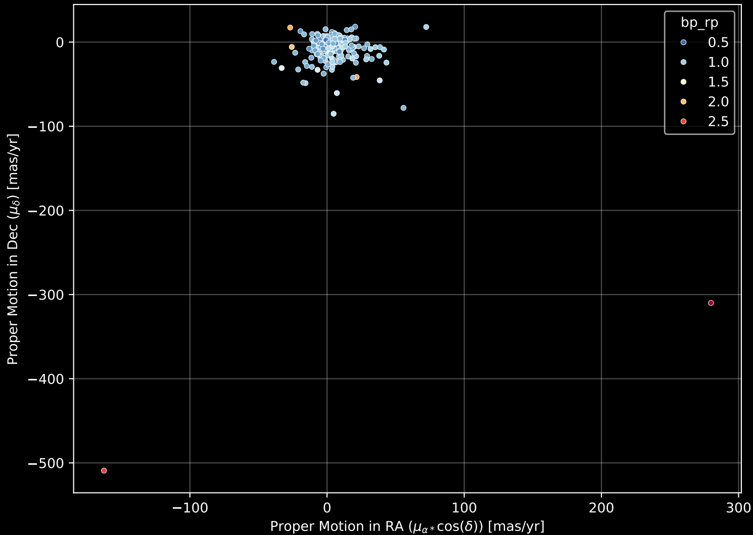
GALAH DR4 Field: [697] Proper Motion Diagram (n= 297)
