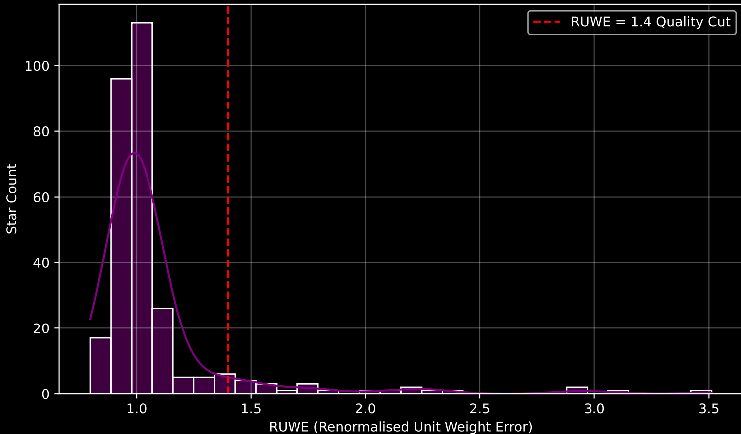
GALAH DR4 Field [697] RUWE Distribution (n= 290)
